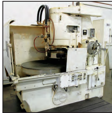
BLANCHARD NO. 18 ROTARY SURFACE GRINDER
