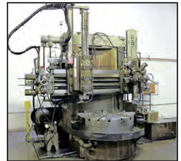
BULLARD CUT MASTER 54" VERTICAL TURRET LATHE
